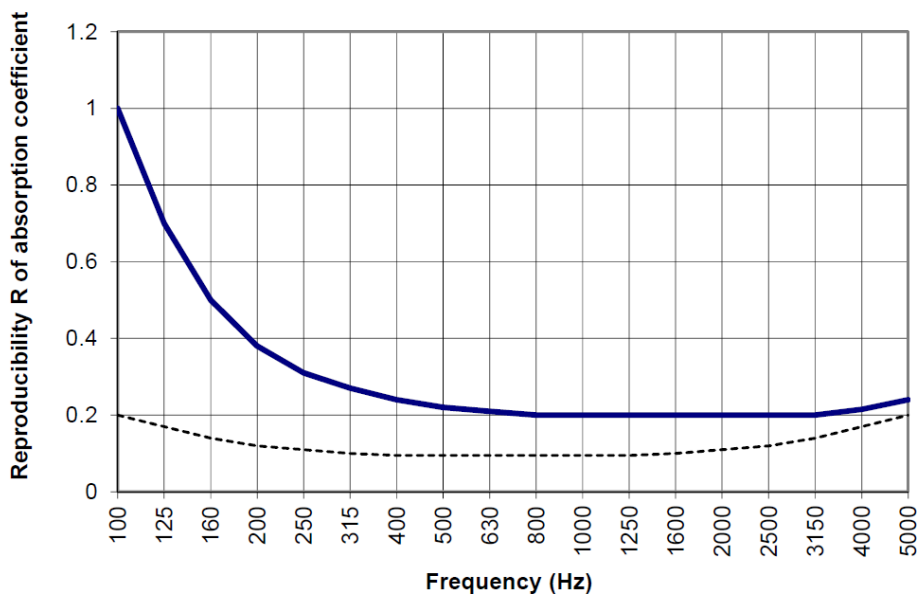
Figure 4.2: Assessment of absorption coefficient reproducibility R from ISO 354-2003(E) – for absorbers with high absorption coefficients ( \alpha_w=1.00 ) in all bands (continuous line) and for absorbers with low absorption coefficients ( \alpha_w=0.05 ) in all bands (dashed line).
