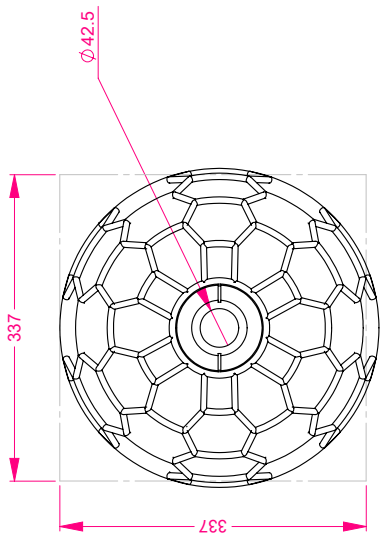
Plan Elevation Scale 1:5
