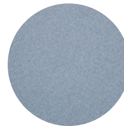
Glacier
