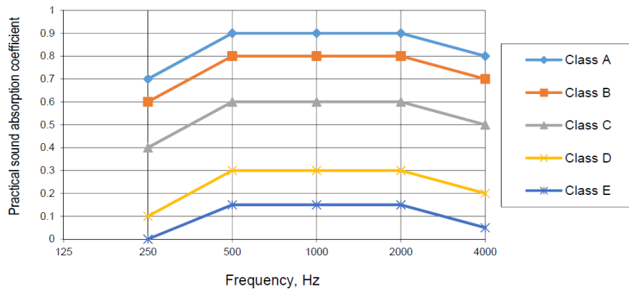
Figure 4.1: The reference curves limiting the different sound absorption classes.
